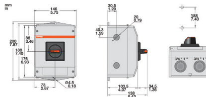
EJM60BSx (enclosure size 2)
