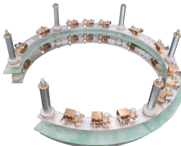
Brush rocker
