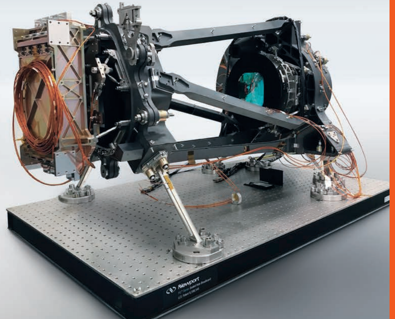
EUCLID NISP INSTRUMENT - IMAGE COURTESY OF LAM
